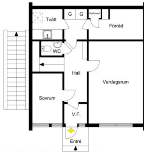
Bottenplan
